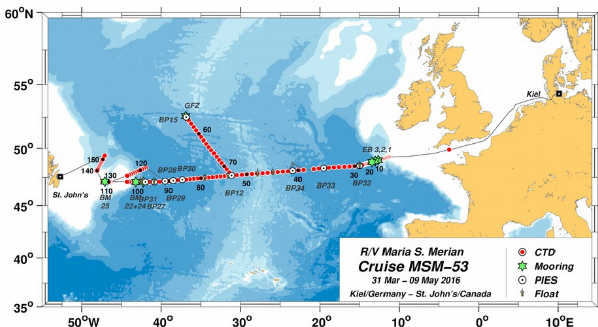
Figure 1. Track of RV MARIA S. MERIAN, cruise MSM-53, and locations of hydrographic profiles.
